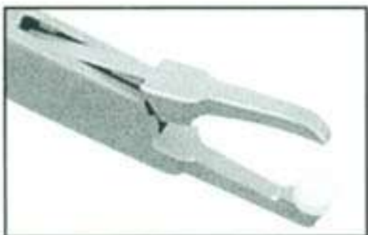
05-167 Band removers curved, Left and Right Curved tips provide easy access and grip of band without excess retractor of cheek or lips
